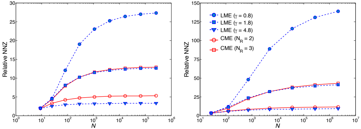
Figure 2: Relative number of nonzeros (NNZ) of sparse matrices as a function of the number of nodes N . The NNZ are scaled by the NNZ of piecewise linear elements on triangles/tetrahedra, which is equivalent to considering N_R = 1 . We show curves of the relative NNZ for CME with N_R = 2, 3 , and for LME with \gamma = 0.8, 1.8, 4.8 and \epsilon_0 = 10^{-6} . Results for uniform grids in 2D (left) and 3D (right) are depicted.
