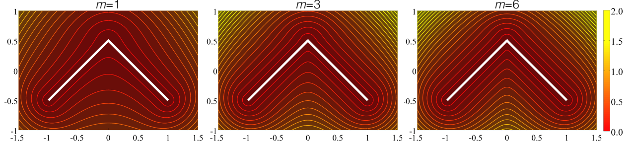
Figure 4: Approximation of the distance function to two line segments by R-equivalence composition (12) for three different values of the normalization parameter m ( m = 1, 3, 6 ).
