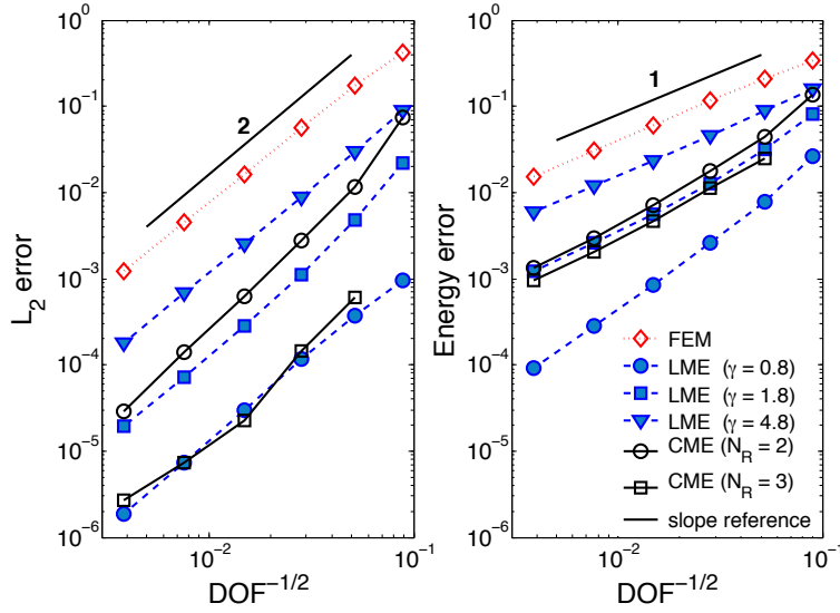
Figure 13: Rates of convergence in the L_2 norm and energy seminorm for linear FE, LME ( \gamma = 0.8, 1.8, 4.8 ; \epsilon_0 = 10^{-6} ) and CME approximants for N_R = 2 ( s = 4, m = 2 ) and N_R = 3 ( s = 3, m = 2 ).
