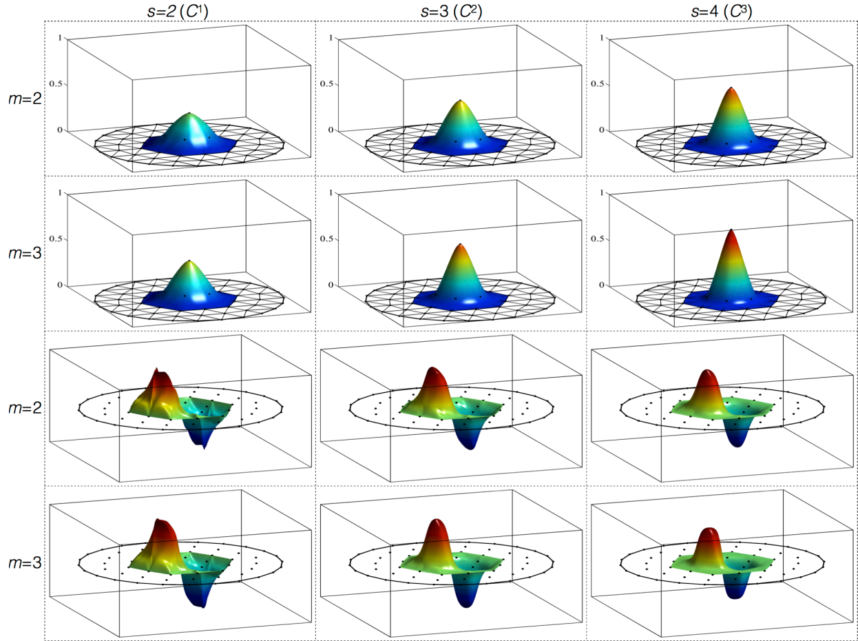
Figure 7: Cell-based max-ent basis functions (arbitrary scale) for several values of the normalization order m and the exponent s . The number of neighbor rings is two ( N_R = 2 ). The top two rows display plots of the basis functions, and the bottom two rows show the derivative along the x -direction.
