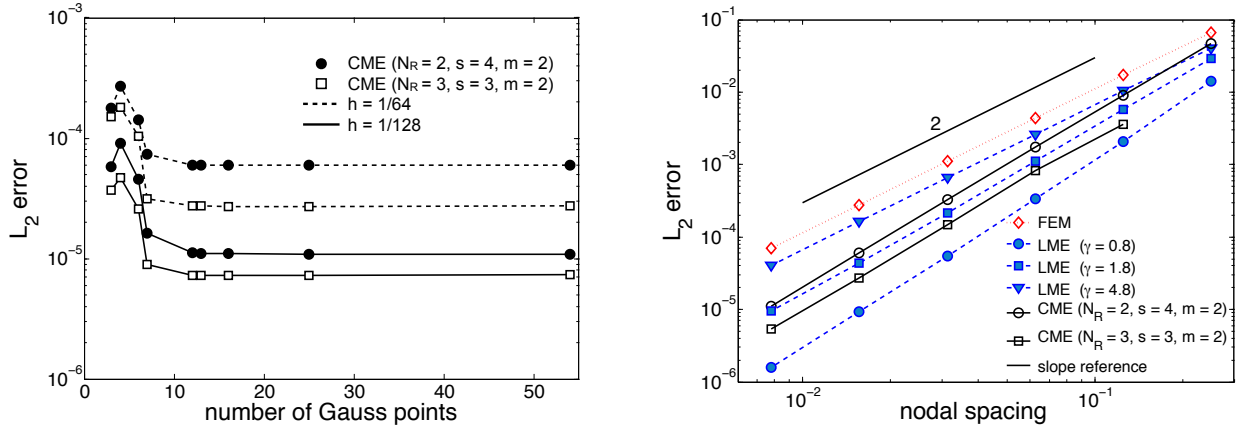
Figure 10: Comparison of FE, LME and CME approximants for a Poisson problem with nonhomogeneous Dirichlet boundary conditions. Left plot shows the error sensitivity with respect to the number of quadrature points for CME approximants. The results on the left panel correspond to two uniform meshes of 65 \times 65 nodes ( h = 1/64 , dashed line) and 129 \times 129 nodes ( h = 1/128 , solid line). The plot on the right shows convergence curves for the relative error in the L_2 norm. Results for CME on the right panel have been obtained with 12 quadrature points.
