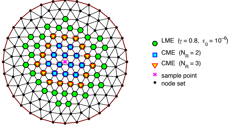
Figure 1: Nearest nodes affecting a given sample point (×) for local and cell-based maximum-entropy approximation schemes.
