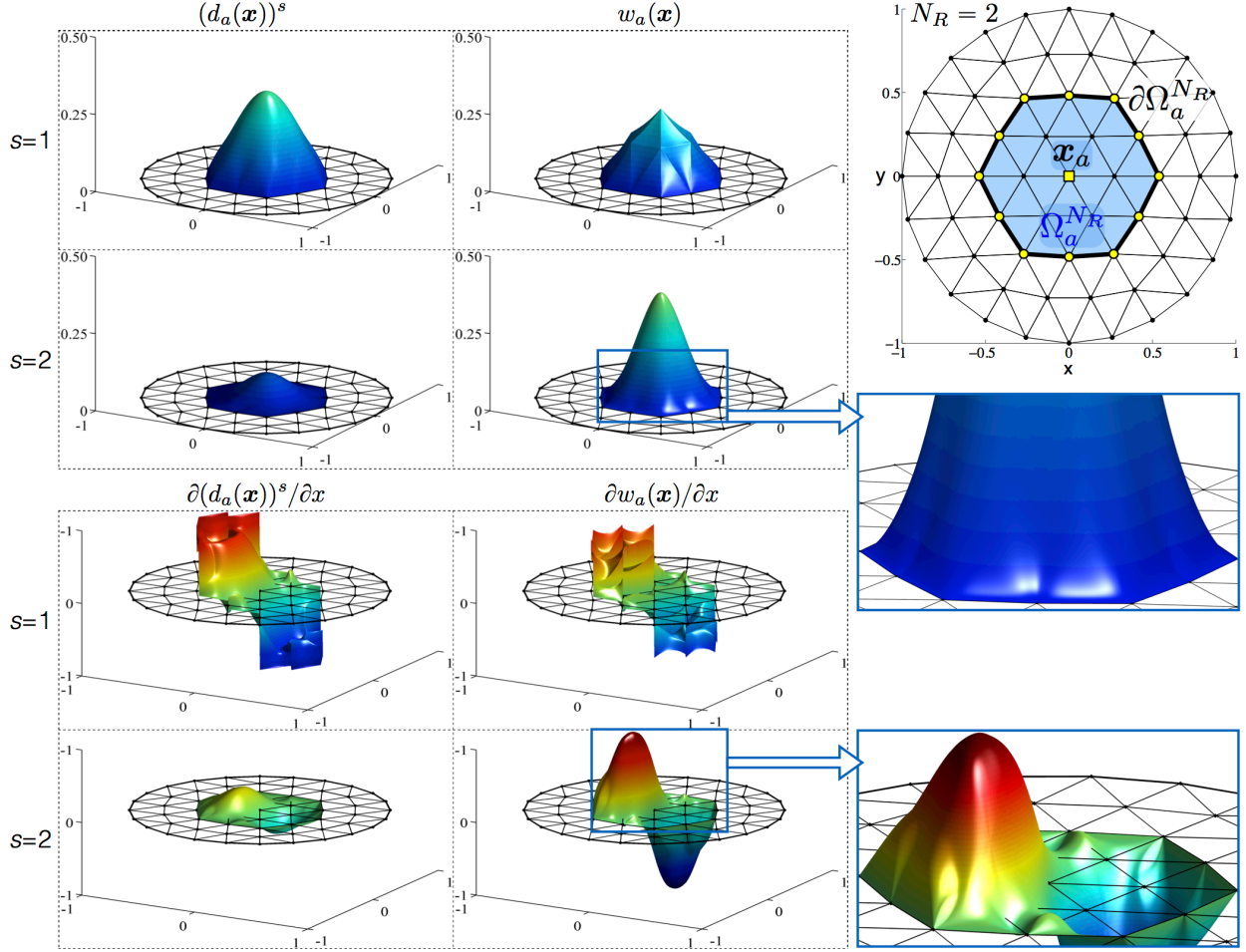
Figure 6: The figure on the upper-right corner shows the mesh considered in this example. The boundary of the polygonal curve \partial\Omega_a^{N_R} for a node \mathbf{x}_a located at the origin ( N_R = 2 ) has been highlighted and is composed of n_a = 12 line segments. The four panels on the top-left show the approximate distance function raised to different powers d_a^s(\mathbf{x}) and the associated prior weight function w_a(\mathbf{x}) (Shepard-form) for the node located at the origin. The approximate distance functions have been obtained by using composition via R-equivalence up to normalization order m = 2 , and powers s = 1, 2 . The bottom four panels display the derivative along the x -direction, where the bulging/creasing effects are apparent close to the vertices of the polygon; see zoom views.
