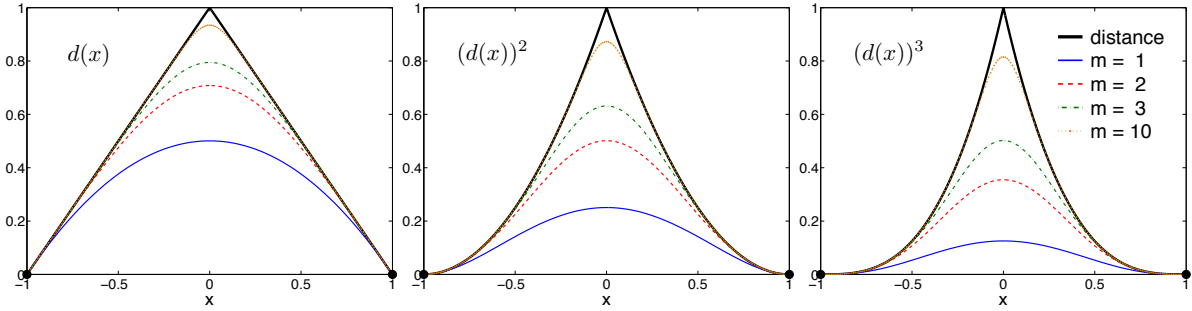
Figure 5: Approximate distance functions d(x) in one-dimension to x = \pm 1 (shown as filled circles) are obtained by composition via R-equivalence up to normalization order m = 1, 2, 3, 10 (left). We also show the powers of the approximate distance functions (d(x))^s for s = 2, 3 (middle, right). In all plots, the exact distance function to a power s is shown as a thick black line.
