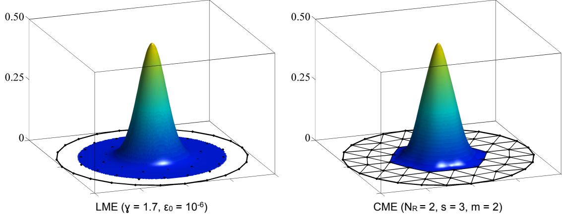
Figure 9: An example of visually similar LME and CME basis functions. The support size of the CME basis function is significantly smaller.
