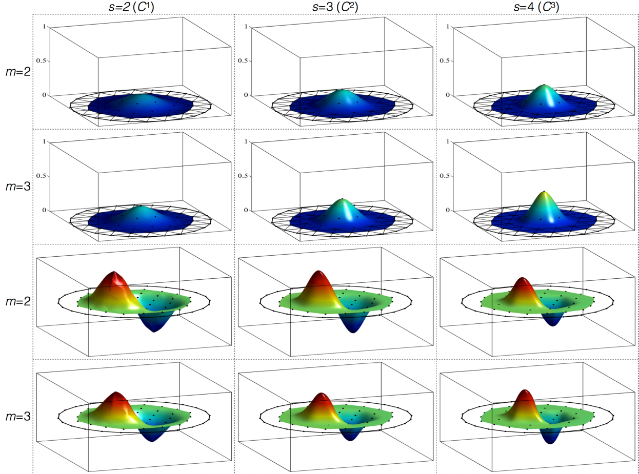
Figure 8: Cell-based max-ent basis functions (arbitrary scale) for several values of the normalization order m and the exponent s . The number of neighbor rings is three ( N_R = 3 ). The top two rows display plots of the basis functions, and the bottom two rows show the derivative along the x -direction.
