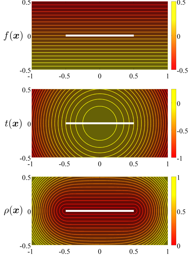
Figure 3: The top plot shows the signed distance function (9) to a line enclosing a segment, the middle plot shows the trimming function (10), and the bottom plot shows the resulting approximation of the distance function (11) to a line segment.
